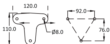
MOUNT DETAILS
