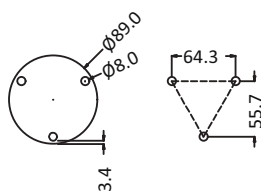
Mount Details
