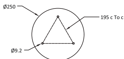
PEDESTAL DETAILS
