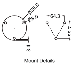
Mount Details
