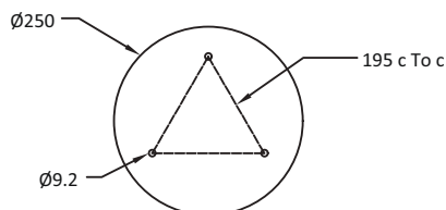
PEDESTAL DETAILS
